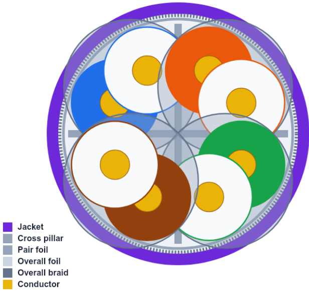
Cross-section diagram S/FTP — braid/foil + cross pillar
