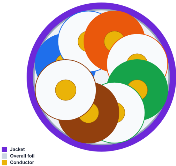
Cross-section diagram F/UTP — overall foil screen
