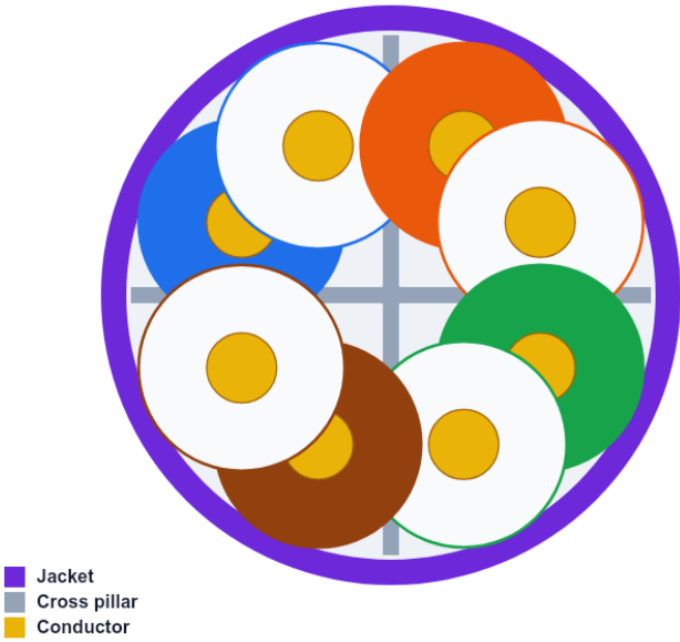
Cross-section diagram U/UTP — with cross pillar
