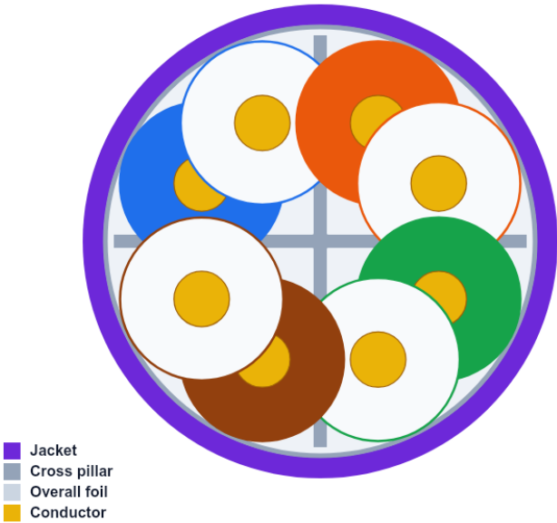
Cross-section diagram F/UTP — overall foil + cross pillar
