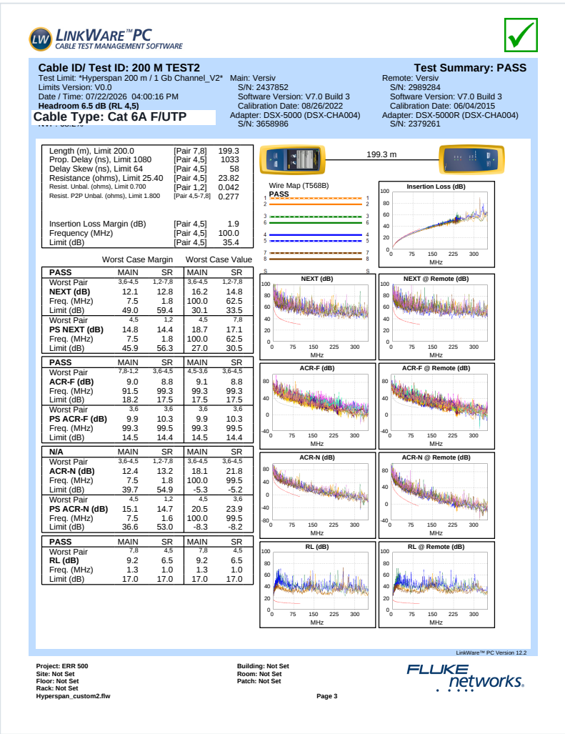
Fluke LinkWare channel test (XR evidence)
