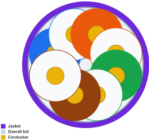
Cross-section diagram F/UTP — overall foil screen
