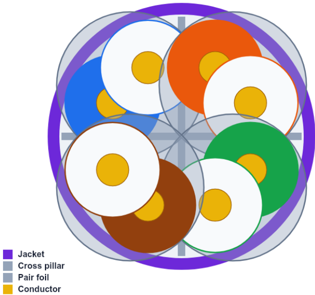
Cross-section diagram U/FTP — foil pairs + cross pillar
