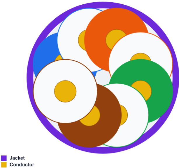
Cross-section diagram U/UTP — unshielded twisted pairs
