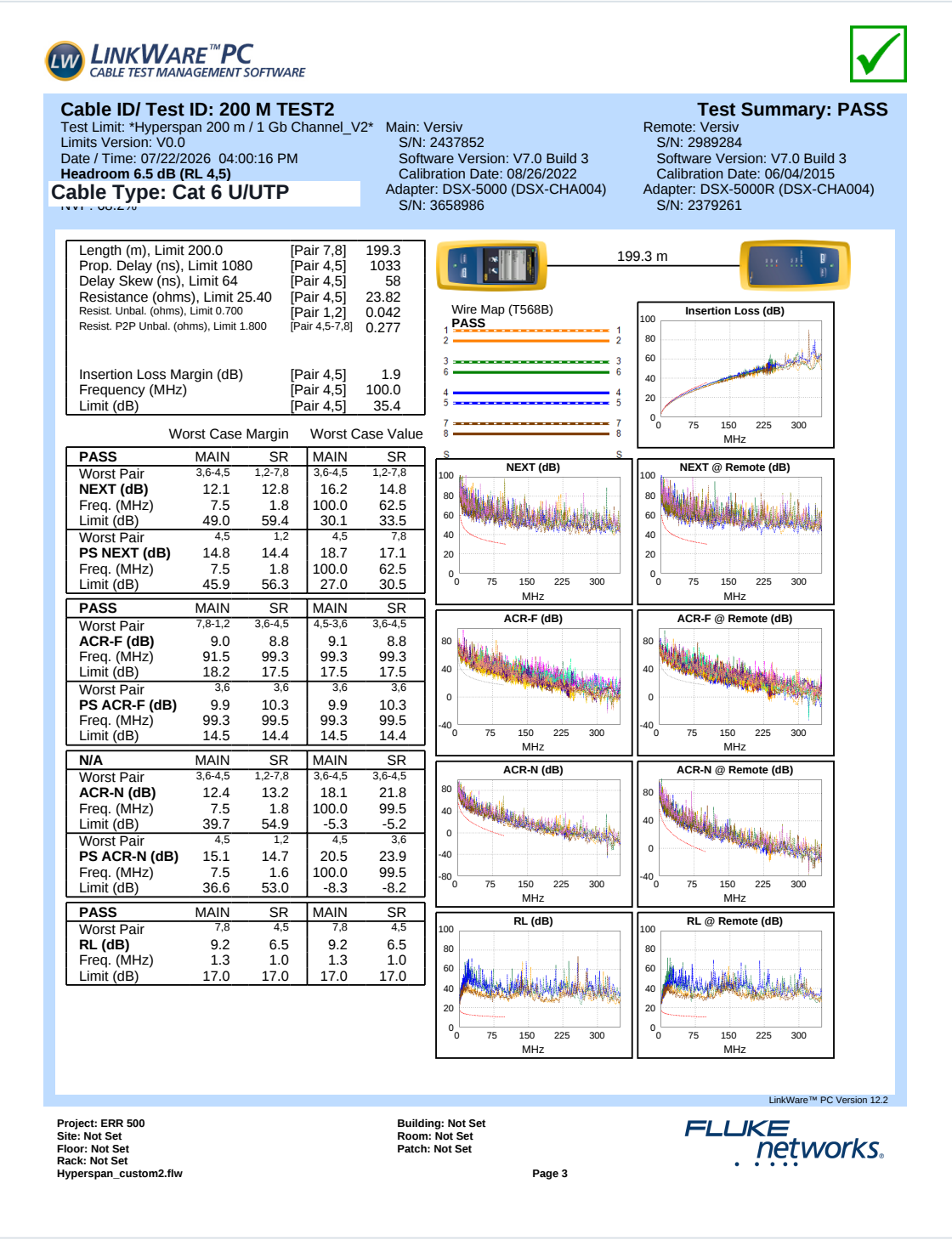
Fluke LinkWare channel test (XR evidence)
